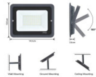
FLOODLIGHT DIMENSION
